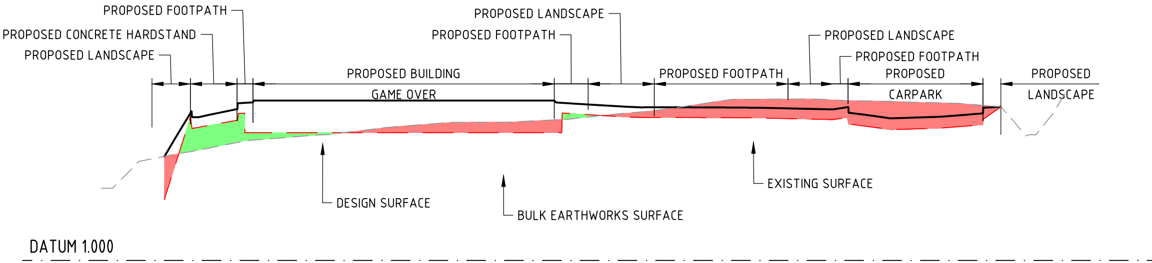
SECTION C H 1500 V 1:100
