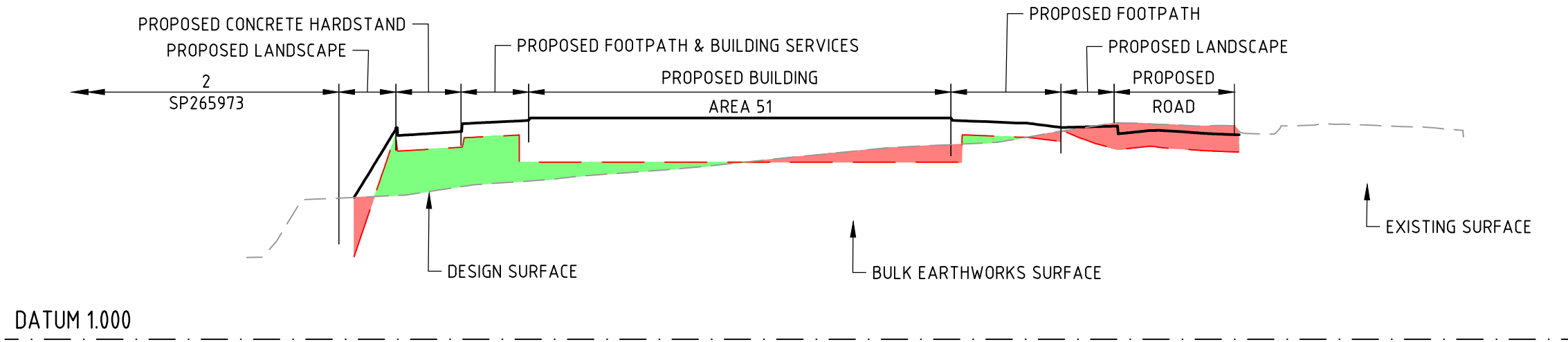
SECTION D H 1500 V 1:100
